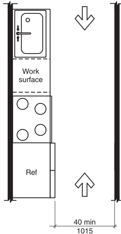
FIGURE 804.2.1(B) PASS-THROUGH KITCHEN CLEARANCE
