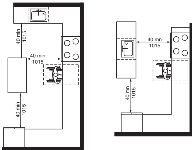
FIGURE 1103.12.1.2(B) U-SHAPED KITCHEN CLEARANCE IN TYPE A UNITS EXCEPTION
