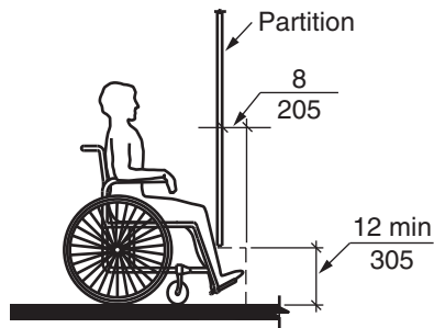
FIGURE 604.9.5(A) TOE CLEARANCE - ELEVATION
