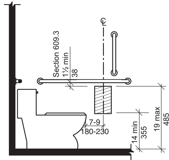
FIGURE 604.11.7(B) CHILDREN'S DISPENSER OUTLET - EXCEPTION
