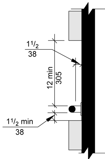
FIGURE 609.3 SPACING OF GRAB BARS
