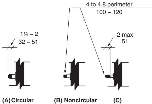
FIGURE 609.2 SIZE OF GRAB BARS
