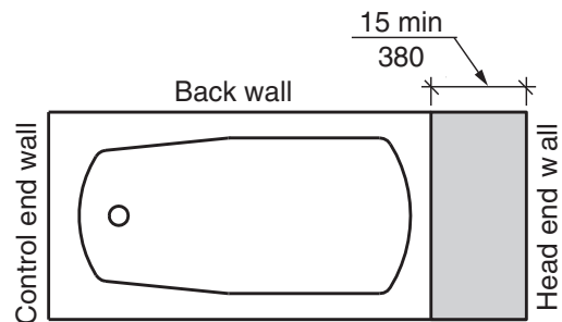
FIGURE 610.2(B) BATHTUB SEATS SEAT PROVIDED AT HEAD END OF TUB
