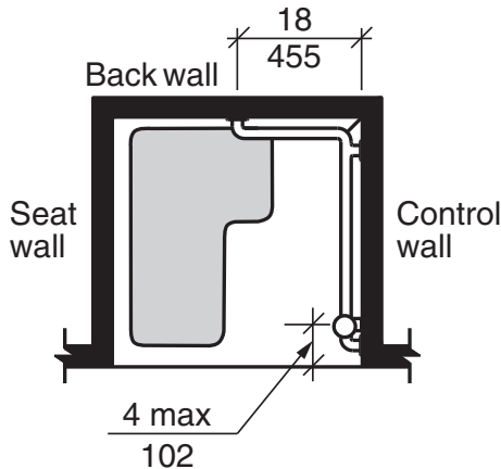
FIGURE 608.3.1(B) GRAB BARS IN TRANSFER-TYPE SHOWER - PLAN
