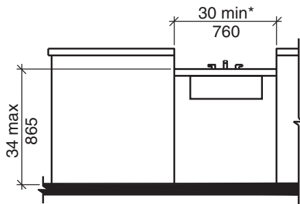
FIGURE 1103.12.4 KITCHEN SINK FOR TYPE A UNITS
