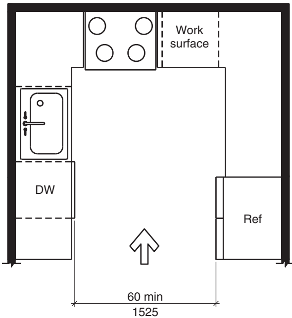
FIGURE 804.2.2(A) U-SHAPED KITCHEN CLEARANCE
