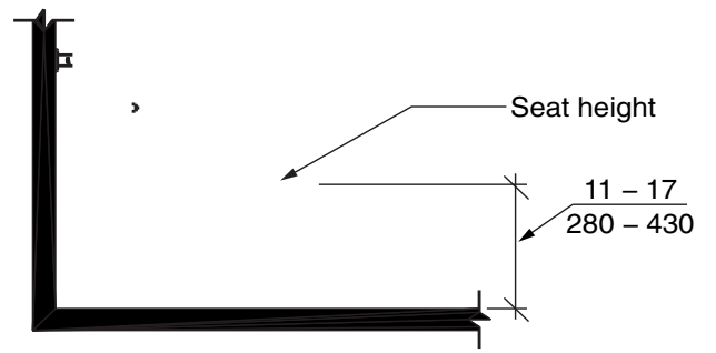
FIGURE 604.11.4 CHILDREN'S WATER CLOSET HEIGHT
