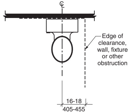
FIGURE 1104.11.3.1.2(A) CLEARANCE AT WATER CLOSETS IN TYPE B UNITS WATER CLOSET LOCATION
