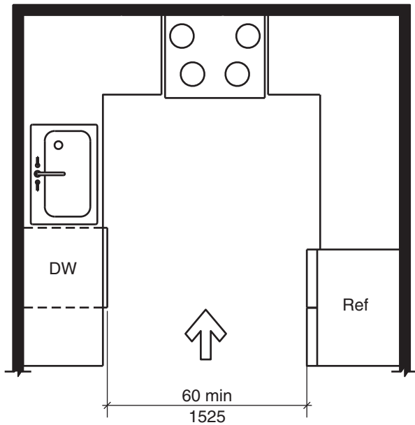
FIGURE 1103.12.1.2(A) U-SHAPED KITCHEN CLEARANCE IN TYPE A UNITS
