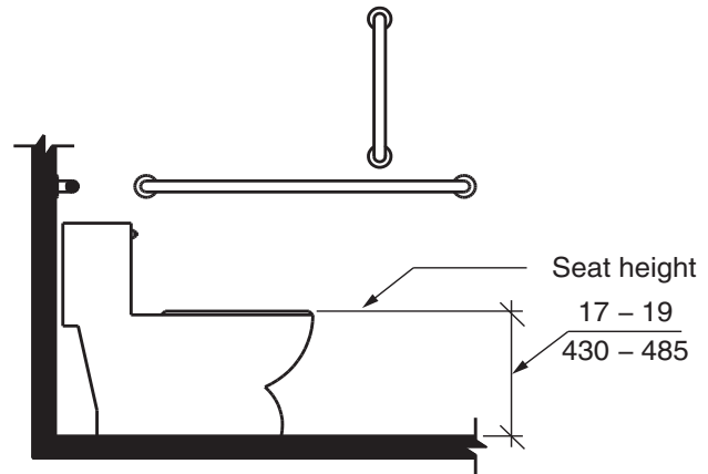
FIGURE 604.4 WATER CLOSET SEAT HEIGHT
