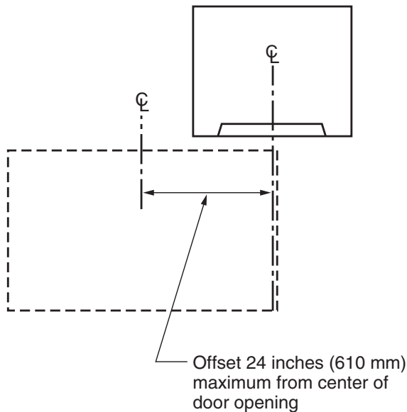
Offset 24 inches (610 mm) maximum from center of door opening FIGURE 611.2(B) CLEAR FLOOR SPACE - FRONT LOADING
