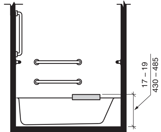
FIGURE 610.2(A) BATHTUB SEATS REMOVABLE IN-TUB SEATS
