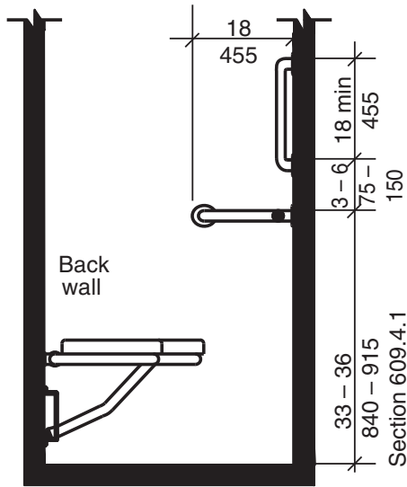
FIGURE 608.3.1(A) GRAB BARS IN TRANSFER-TYPE SHOWER - ELEVATION
