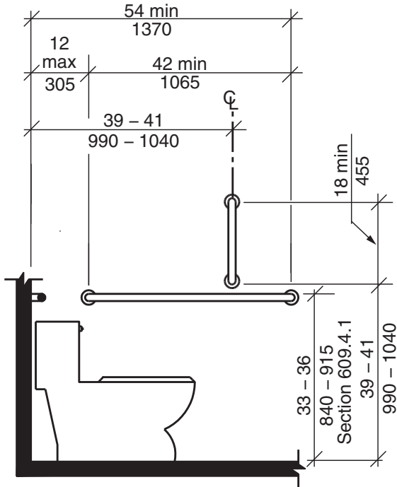
Note: For children's dimensions see Fig. 609.4.2 FIGURE 604.5.1
