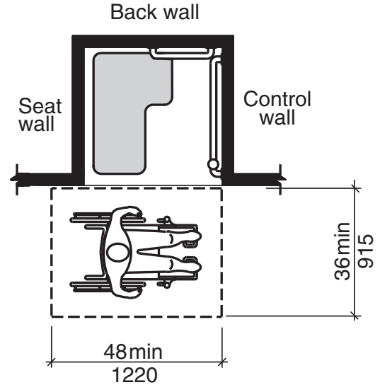
FIGURE 608.2.1.2(C) TRANSFER-TYPE SHOWER COMPARTMENT CLEARANCES EXISTING BUILDINGS
