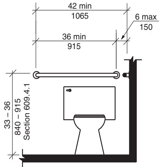
Note: For children's dimensions see Fig. 609.4.2
