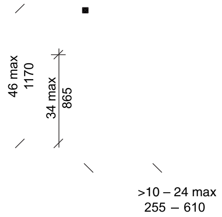
FIGURE 308.3.2(B) OBSTRUCTED HIGH SIDE REACH
