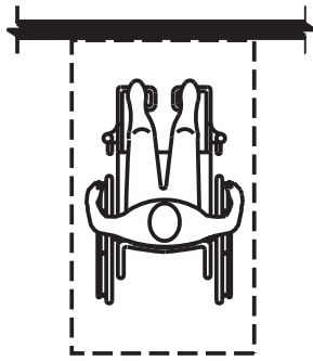
FIGURE 305.5(A) POSITION OF CLEAR FLOOR SPACE - FORWARD
