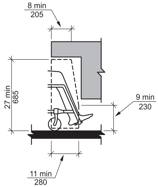
FIGURE 306.3(A) KNEE CLEARANCE - ELEVATION
