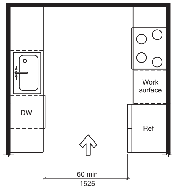
FIGURE 804.2.2(B) U-SHAPED KITCHEN CLEARANCE
