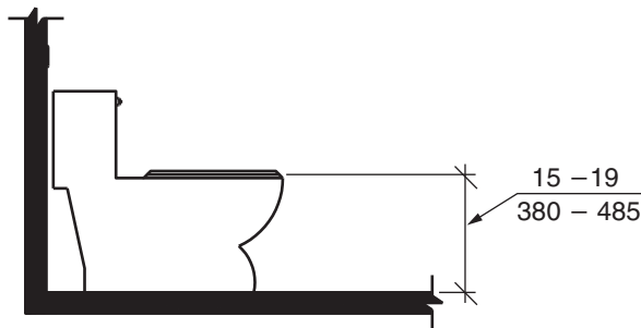
FIGURE 1103.11.2.4(D) WATER CLOSETS IN TYPE A UNITS - WATER CLOSET SEAT HEIGHT
