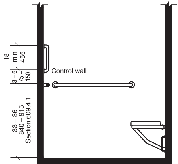
FIGURE 608.3.2(A) GRAB BARS IN STANDARD ROLL-IN-TYPE SHOWER ELEVATION
